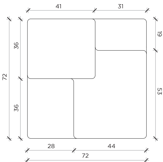
FRONTE | FRONT
